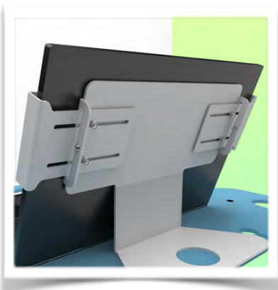
Secure laptop holder Part Number: WM555.9017
