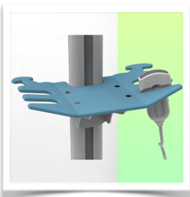
Gel holder Fixation on Din rail 10 x 25 mm Part Number: WM555.6063
