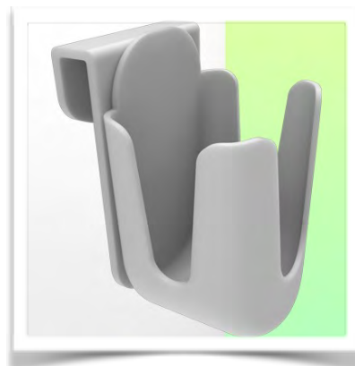
Mouse Holder 10 x 25 mm Din rail mounting Part Number: WM555.6024
