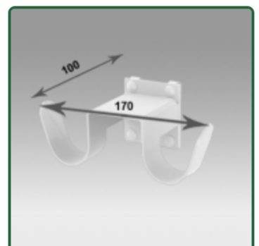
Double cable hooks for vertical slide rail mounting Part Number: 999.156
