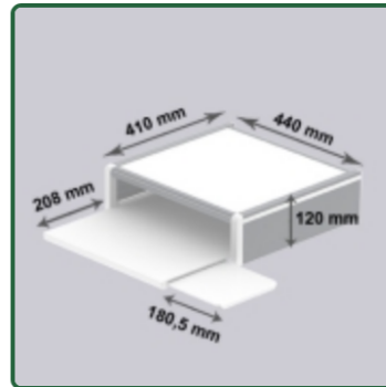
Drawer and Keyboard Stand Vertical Slide Rail Mounting Part Number: 999.151
