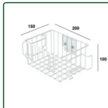
Small service basket, vertical slide rail mounting Part Number: 999.155
