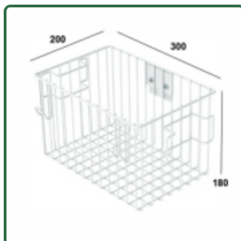
Large service basket, vertical slide rail mounting Part Number: 999.154
