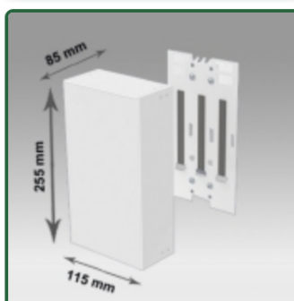
Electrical power supply box 255 x 115 x 85 mm
