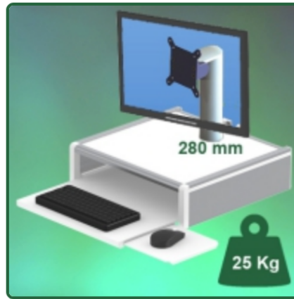
Medical Monitor Console, Height 280 mm, Keyboard Platform Medical Column Mount Part Number: 991.865
