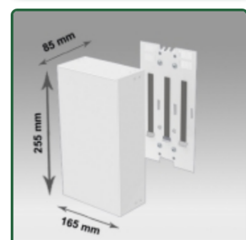
Electrical power supply box 255 x 165 x 85 mm
