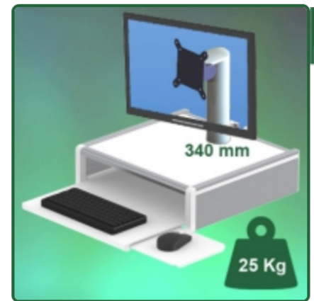
Medical Monitor Console, Height 340 mm, Keyboard Platform Medical Column Mount Part Number: 991.866
