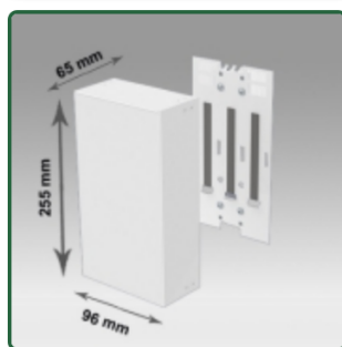
Electrical power supply box 255 x 96 x 65 mm Part Number: 999.166
