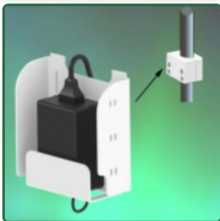
Power supply stand Mounting on Pole 25 mm
