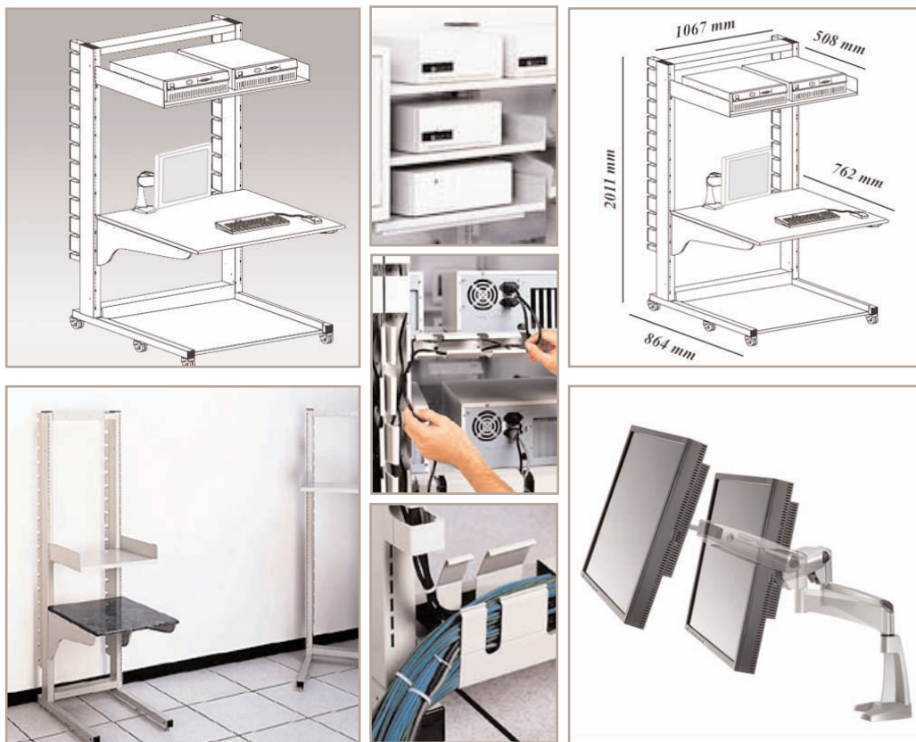
Console Rack Lan 42" (1067 mm)
